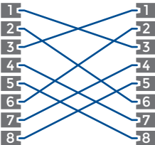
Cross-over Gigabit T568 B IEEE 802.3
